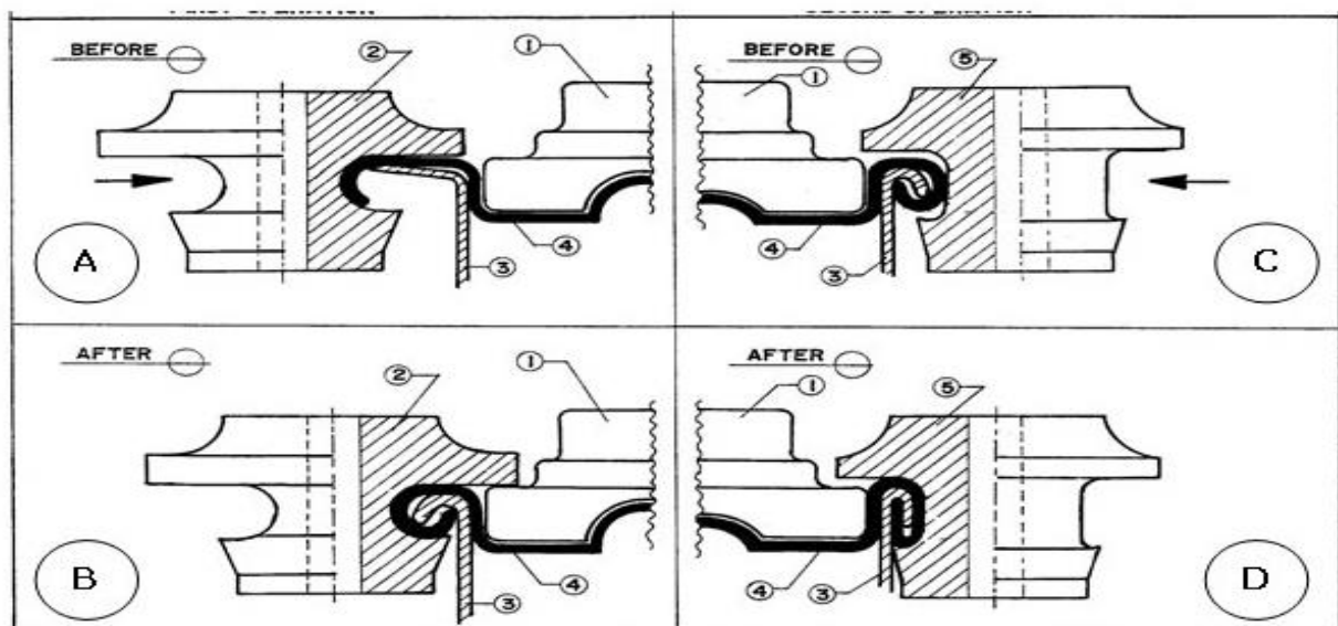
Fig. 5 Example of execution of the double countersink.
