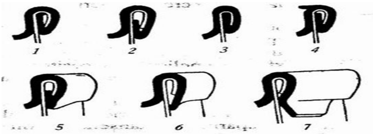
Fig 4. Forms of double countersink
