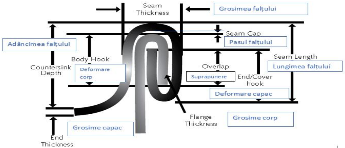
Fig 3: The elements of the normal double countersink 2
